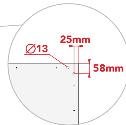
Top Shelf Access Holes Same measurements for each corner
