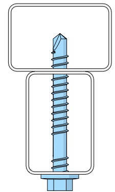
Shelf RHS Tee Section Stiffner
