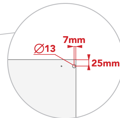
Internal Shelves Access Holes Same measurements for each corner
